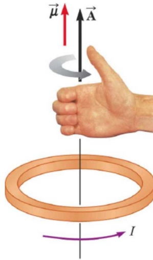
Figure The right-hand rule for the magnetic moment
