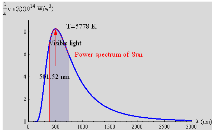
Fig. Power spectrum of sun. cu(\lambda)/4 ( \text{W/m}^3 ) vs \lambda (nm). T = 5778 \text{ K} . The peak wavelength is 501.52 nm according to the Wien's displacement law.
