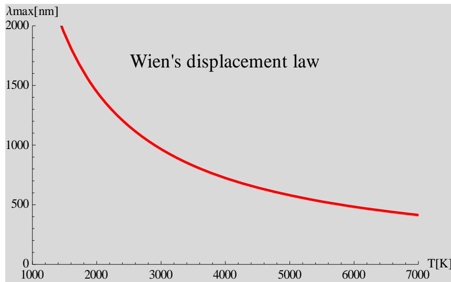
Fig. Wien's displacement law. The peak wavelength vs temperature T(\text{K}) .
