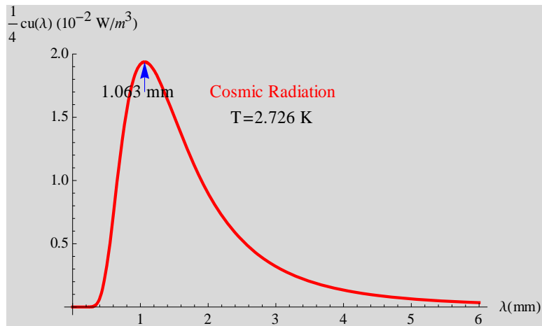
Fig. Power spectrum of cosmic blackbody radiation at T = 2.726 \text{ K} . The peak wavelength is 1.063 mm (Wien's displacement law).
