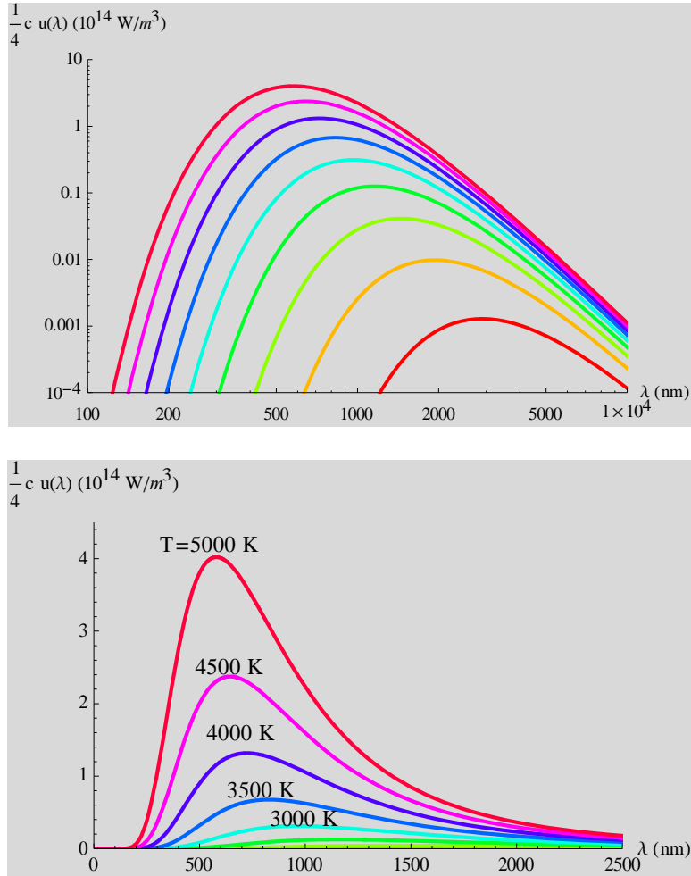
Fig. (a) and (b) cu(\lambda)/4 ( \text{W/m}^3 ) vs \lambda (nm) for the Planck's law. T = 1000 K (red), 1500 K, 2000 K, 2500 K, 3000 K (blue), 3500 K, 4000 K (purple), 4500 K, and 5000 K. The peak shifts to the higher wavelength side as T decreases according to the Wien's displacement law.
