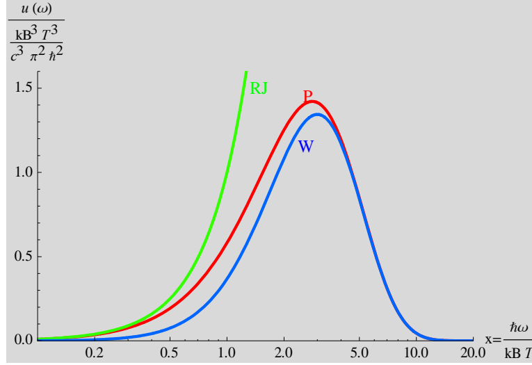
Fig. Scaling plot of Planck's law. Wien's law, and Rayleigh-Jean's law.
