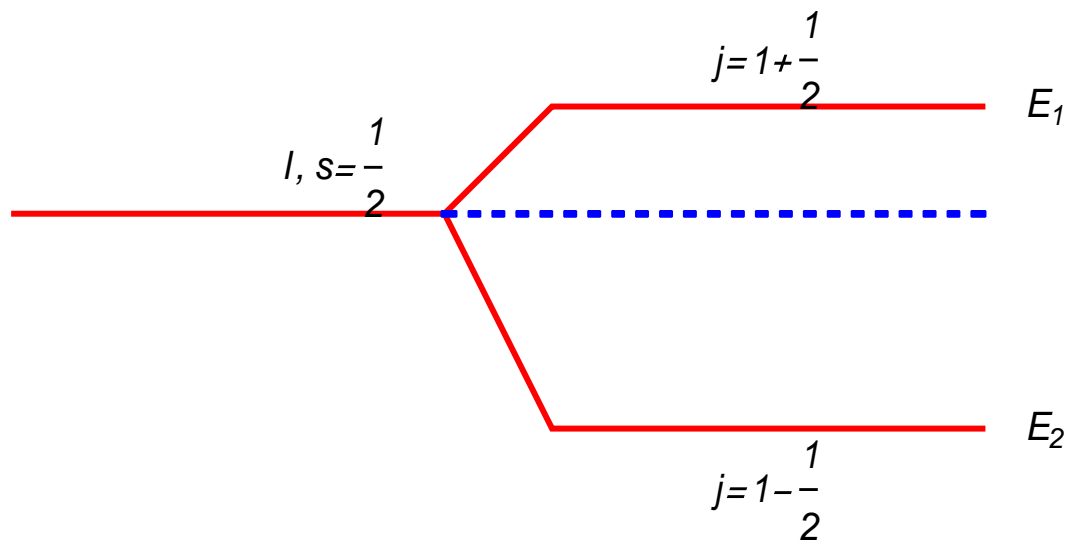
Fig. Splitting of the energy level due to the spin-orbit interaction. E_1 = \frac{l\xi\hbar^2}{2} . E_2 = -\frac{(l+1)\xi\hbar^2}{2} . This splitting is independent of the quantum number m .
