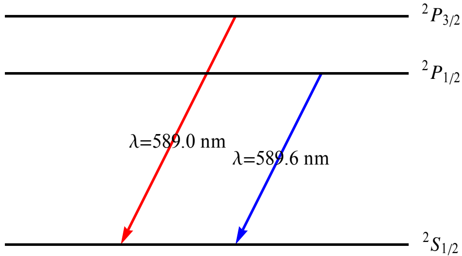
Fig. 3^2P_{3/2} ( j = 3/2, l = 1, s = 1/2 ). 3^2P_{1/2} ( j = 1/2, l = 1, s = 1/2 ). 3^2S_{1/2} ( j = 1/2, l = 0, s = 1/2 ). The splitting of the energy levels ( 3^2P_{3/2} and the 3^2P_{1/2} ) is due to the spin-orbit interaction. The D 1 line (denoted by blue line). The D 2 line (denoted by red line).
