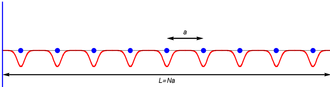
Fig. Periodic lattice of lattice constant a . The form of potential energy of an electron in a one-dimensional lattice. The positions of the ion cores are indicated by the points (blue solid circles) with the separation a (lattice constant).
