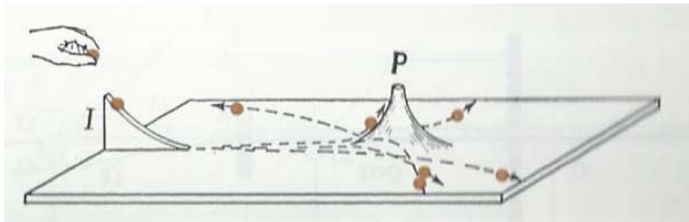
Fig. Mechanical model of an atomic nucleus for demonstrating Rutherford scattering
