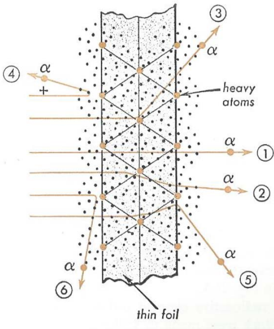
Fig. Diagram of the deflection of an \alpha particle by a nucleus: Rutherford scattering
