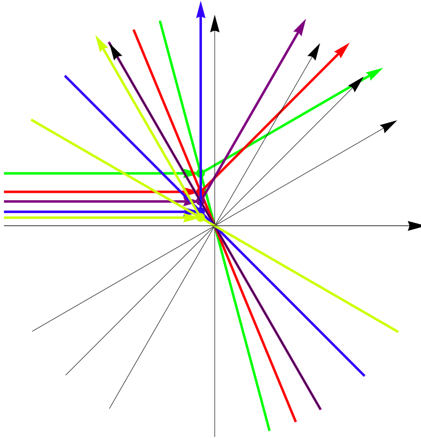
Fig. Schematic diagram for the Rutherford scattering where \theta is varied as a parameter. The relation between the impact parameter b and the scattering angle \theta . As b increases, the angle \theta decreases (smaller angle).
