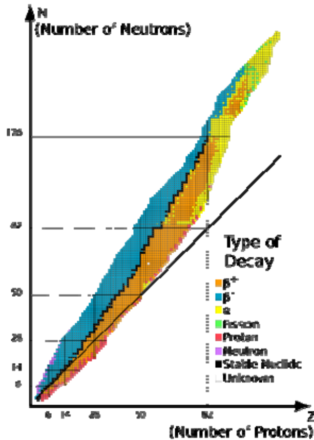
Fig. Graph of isotope stability http://en.wikipedia.org/wiki/Magic_number_%28physics%29
