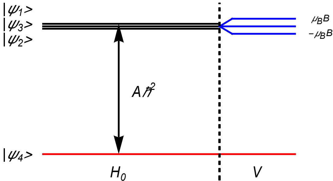
Fig. The states |\psi_1\rangle , |\psi_3\rangle , and |\psi_2\rangle are degenerate states with the energy \frac{A\hbar^2}{4} . The state |\psi_4\rangle is a nondegenerate state with -\frac{3A\hbar^2}{4} . Under the perturbation of V (the first order), the degenerate states are separated into nondegenerate state.
