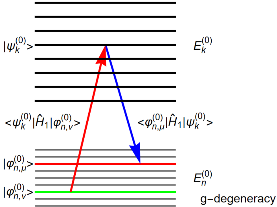
Fig. The second order perturbation for the degenerate state ( g -degeneracy). Matrix elements \langle \varphi_{n,\mu}^{(0)} | \hat{H}_1 | \psi_k^{(0)} \rangle and \langle \psi_k^{(0)} | \hat{H}_1 | \varphi_{n,\nu}^{(0)} \rangle for this system. E_n^{(0)} \neq E_k^{(0)} . The factor 1/[E_n^{(0)} - E_k^{(0)}] is necessary for the final result.
