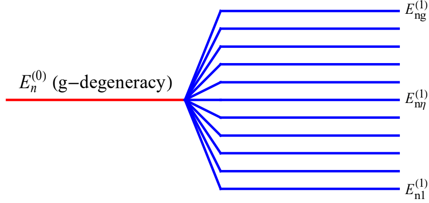
Fig. Energy level with the g -degeneracy for the unperturbed system ( \hat{H}_0 ). Under the perturbation ( \hat{H}_1 ), the energy level splits into various energy levels.
