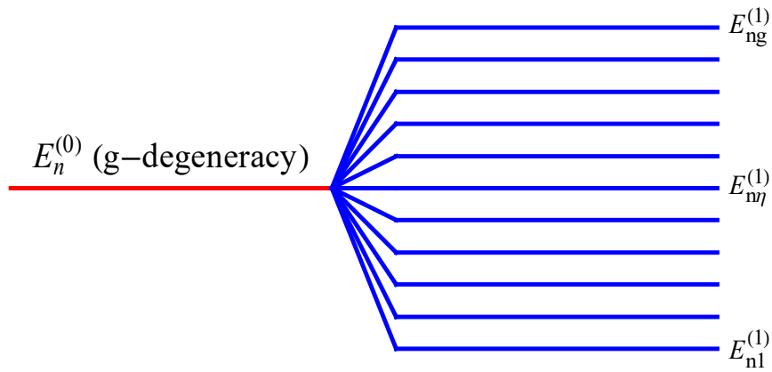
Fig. g -degeneracy. |\varphi_{n,\mu}^{(0)}\rangle state ( \mu = 1, 2, \dots, g ) with the same energy E_n^{(0)}
