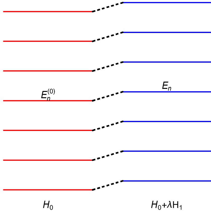
Fig. Shift of the energy levels when the perturbed Hamiltonian ( \lambda\hat{H}_1 ) is added to the system.
