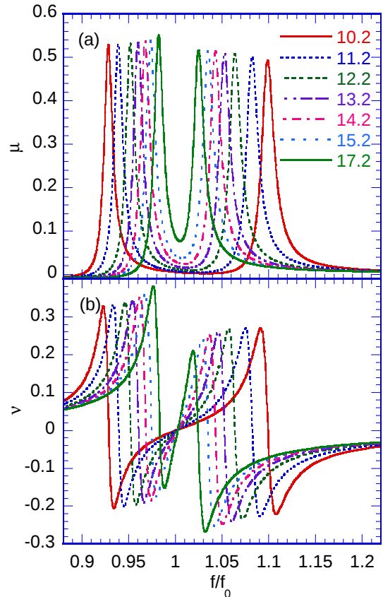
FIG. 4: (Color online) Experimental plot of (a) the real part ( \mu ) and (b) the imaginary part ( \nu ) as a function of x (= f/f_0) (in the frequency scan). The distance d between the centers of two coils is changed as a parameter. d = 10.2 cm - 17.2 cm. f_0 = 2850 Hz. Q = 151.5 .
