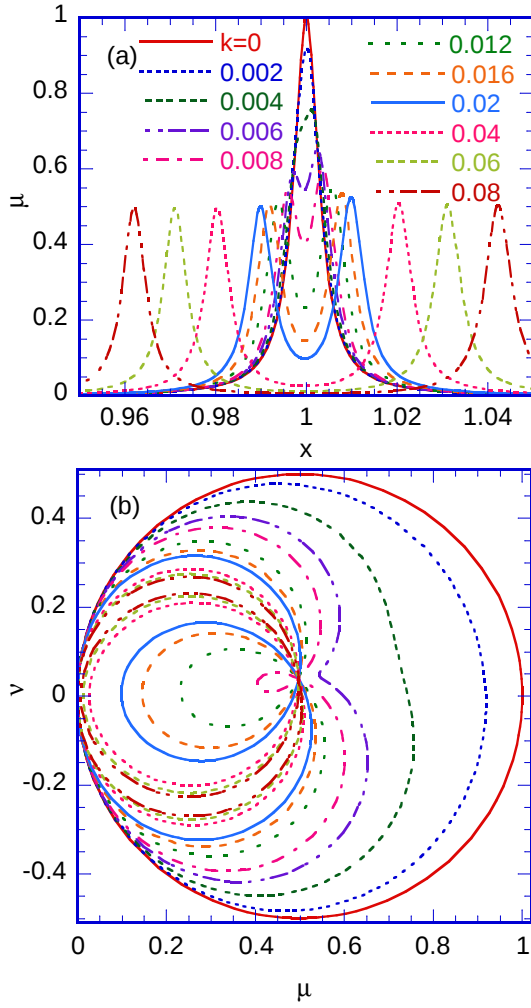
FIG. 9: (Color online) (a) Simulation plot of the real part ( \mu ) as a function of x , where Q = 151.5 and L_1 = 0.8207 H and L_2 = 0.8215 H (the symmetric configuration). (b) The trajectory of the point (\mu, \nu) for Q = 151.5 , L_1 = 0.8207 H and L_2 = 0.8215 H, when x is varied from x = 0 to \infty . The coupling constant k is changes as a parameter: k = 0 - 0.08 .
