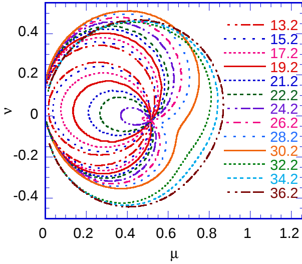
FIG. 6: (Color online) Experimental trajectories of the point ( \mu, \nu ) for Q = 151.5 , when x ( = f/f_0 ) is varied from x = 0.947 ( f = 2700 Hz) to 1.053 ( f = 3000 Hz). f_0 = 2850 Hz. The distance is changed as a parameter: d = 13.2 - 36.2 cm. The deviation of the experimental trajectories from the ideal one as shown in Fig. 3(c) is partly due to the asymmetric configuration ( L_1 is slightly larger than L_2 ).
