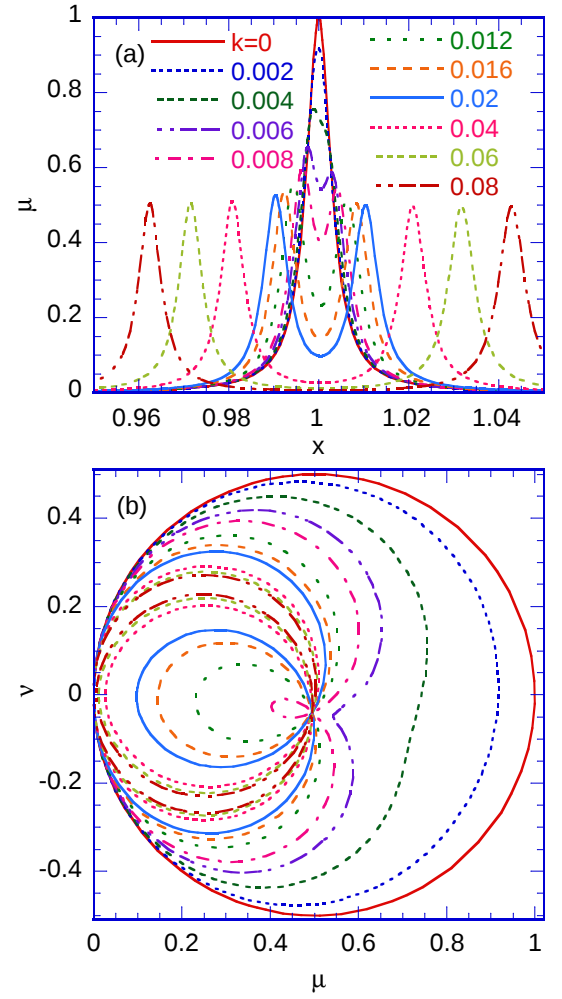
FIG. 10: (Color online) (a) Simulation plot of the real part ( \mu ) as a function of x , where Q = 151.5 and L_1 = 0.8207 H and L_2 = 0.8198 H. The coupling constant k is changed as a parameter: k = 0 - 0.08 . (b) Typical trajectory denoted by the point (\mu, \nu) for Q = 151.5 , when x is varied from x = 0 to \infty . The coupling constant k is changes as a parameter: k = 0 - 0.08 .
