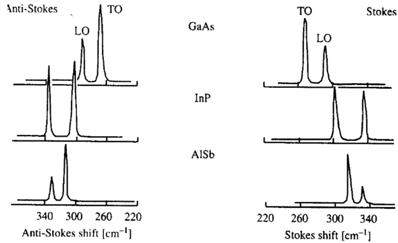
Fig. Raman spectra of three zinc-blende-type semiconductors showing the TO and LO phonons in both Stokes and anti-Stokes scattering. (M.S. Dresselhaus, Solid State
