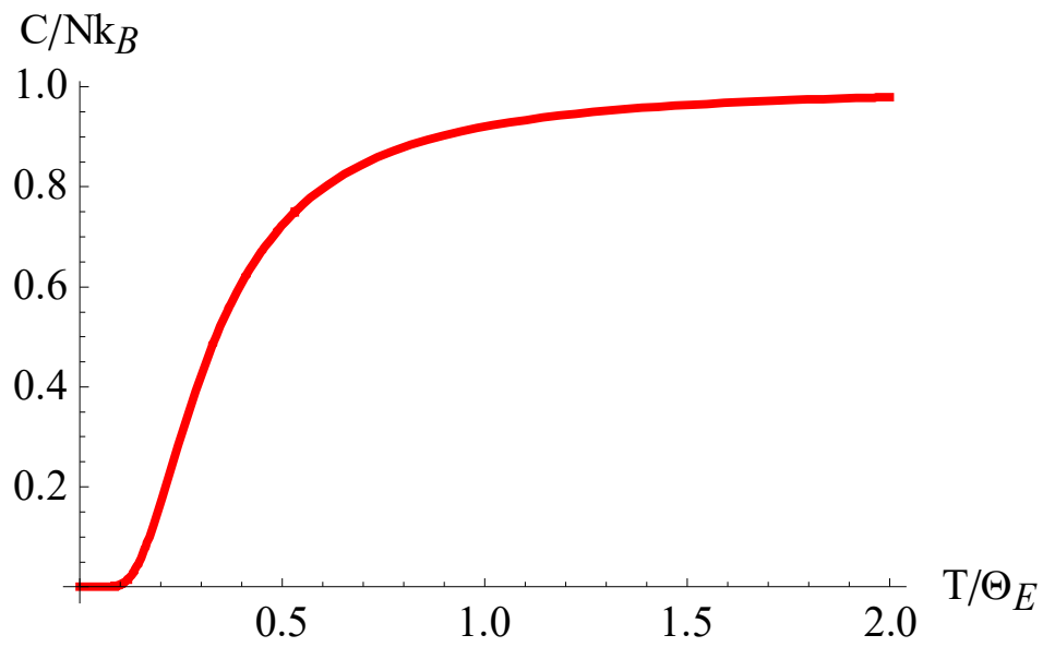
Fig. Heat capacity for the Einstein model.
