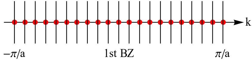
Fig. First Brillouin zone. There are N states for |k| \leq \pi/a .
