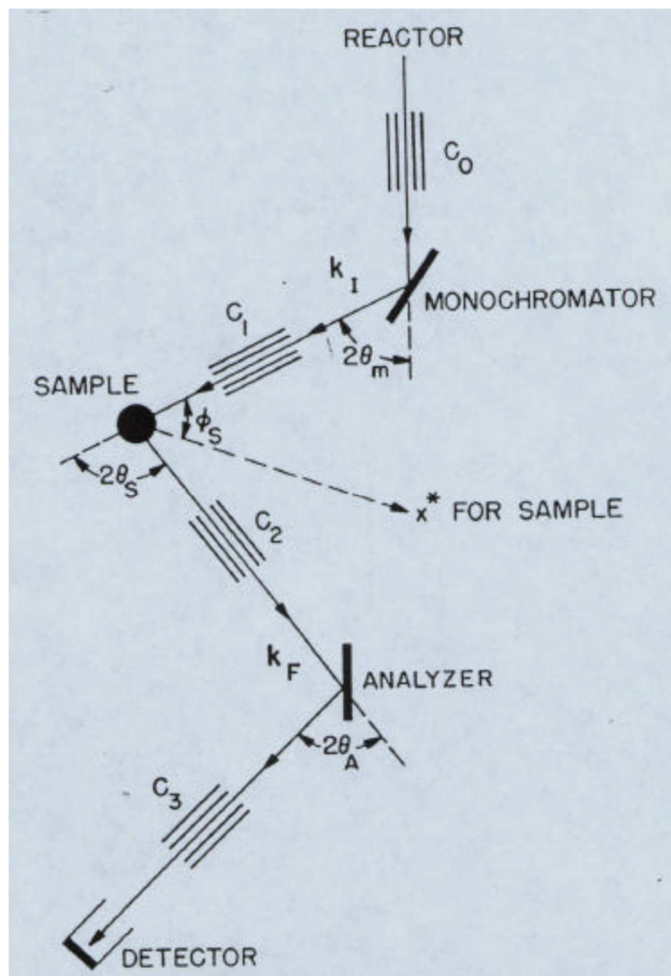
Fig. Schematic diagram for the triple-axis spectrometer for the measurement of inelastic neutron scattering.
