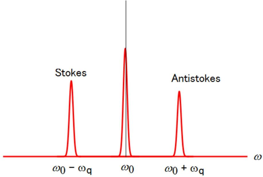
Fig. Schematic diagram of Raman scattering. Unshifted Rayleigh line ( \omega_0 ). Stokes line (emission, \omega_0 - \omega_q ) and anti-Stokes line (absorption, \omega_0 + \omega_q ). The ratio of the Stokes to anti-Stokes can be used to estimate the temperature of the phonon system
