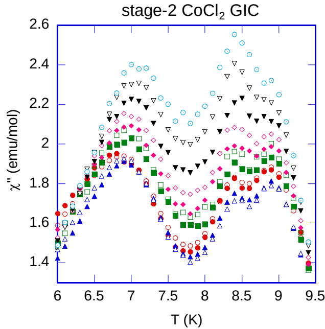
Fig.7 T dependence of the absorption \chi''(\omega, T) of stage-2 CoCl 2 GIC at various frequencies: f = 0.1 - 1000 Hz . h = 50 mOe. h \perp c . The c axis is perpendicular to the basal plane of the system. H = 0 (no external DC magnetic field). Ref.[23].
