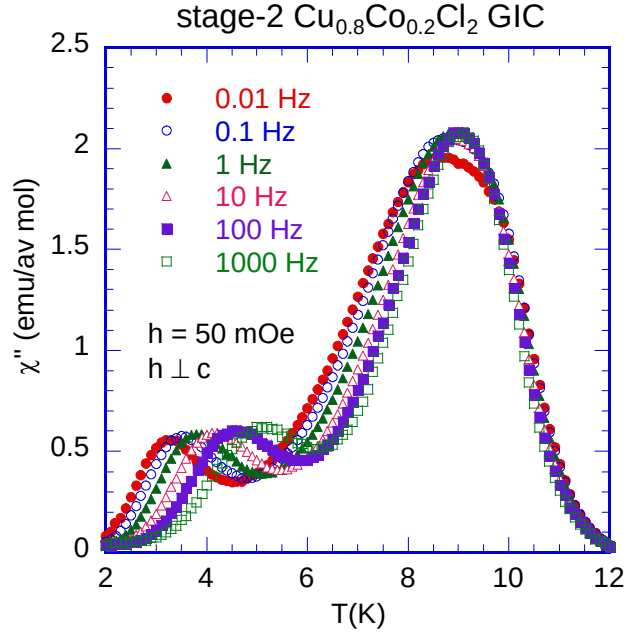
Fig.9 T dependence of the absorption \chi''(\omega, T) of stage-2 \text{Cu}_{0.8}\text{Co}_{0.2}\text{Cl}_2 GIC (graphite intercalation compound) at various frequencies: f = 0.01 - 1000 Hz . h = 50 mOe. h \perp c . The c axis is perpendicular to the basal plane of the system. H = 0 (no external DC magnetic field). Ref.[25].
