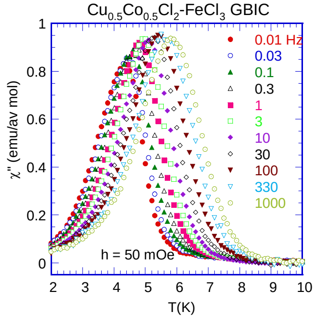
Fig.8 T dependence of the absorption \chi''(\omega, T) of \text{Cu}_{0.5}\text{Co}_{0.5}\text{Cl}_2\text{-FeCl}_3 GBIC at various frequencies: f = 0.01 - 1000 Hz . h = 50 mOe. h \perp c . The c axis is perpendicular to the basal plane of the system. H = 0 (no external DC magnetic field). Ref.[24].
