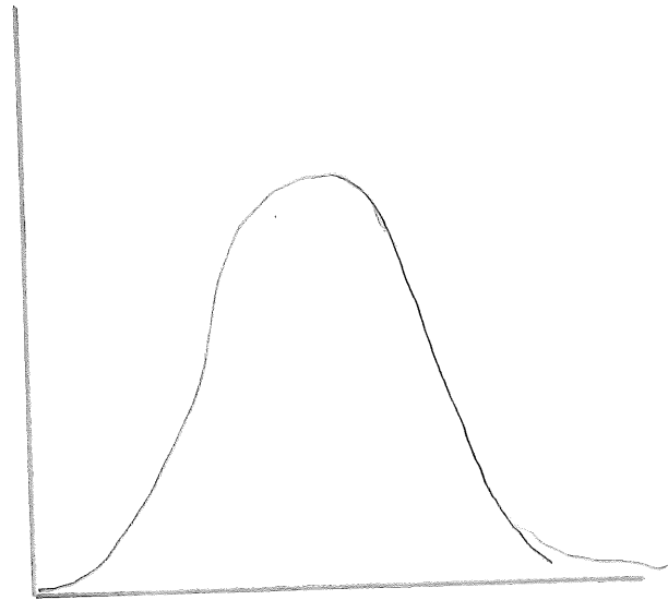
Normal distribution
