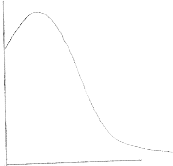
Poisson distribution:
