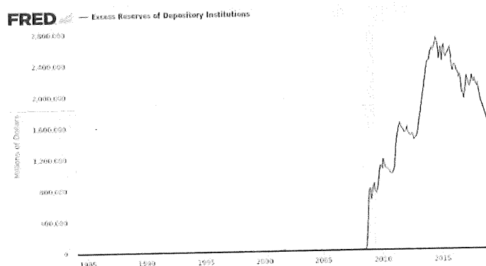
Figure 4 Excess Reserves
