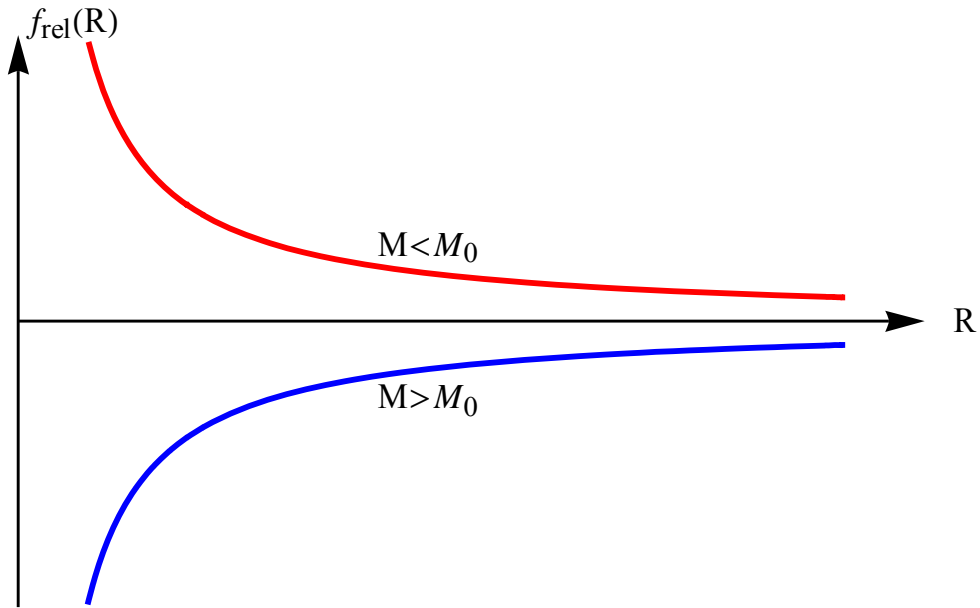
Fig. Schematic plot of f_{rel}(R) vs R for M > M_0 and M < M_0 . When M = M_0 , f_{rel}(R) = 0 .
