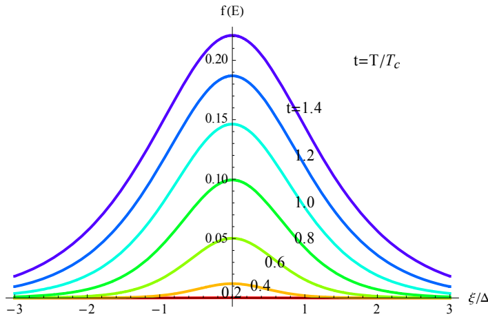
Fig. Plot of f(E) as a function of \xi/\Delta . t is the reduced temperature; t = T/T_c . t = 0.2, 0.4, 0.6, 0.8, 1.0, 1.2, and 1.4 .
