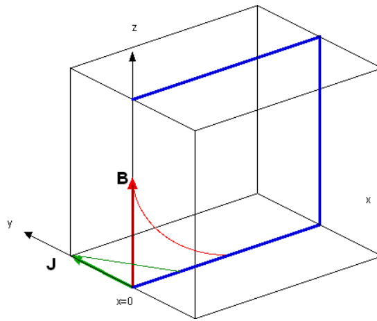
Fig. The distribution of the magnetic induction B(x) (along the z axis) and the current density (along the y axis) near the boundary between the normal phase and the superconducting phase. The plane with x = 0 is the boundary.
