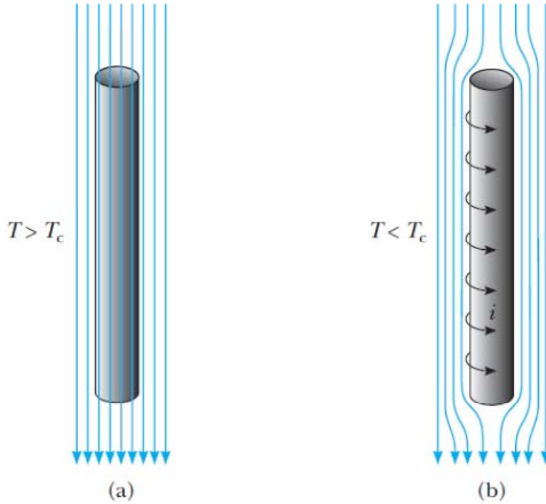
Fig. For T < T_c , the surface current flows near the surface, leading to the cancellation of the external magnetic field. Meissner effect.
