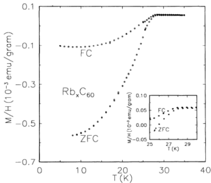
Fig. Magnetization of a sample of nominal composition \text{Rb}_3\text{C}_{60} . The data labeled ZFC were obtained upon warming in a field of 2 Oe, after cooling the sample in zero applied field. The FC data were obtained by cooling the sample in 2 Oe, illustrating flux expulsion.
