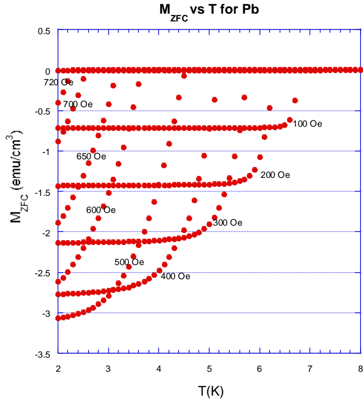
Fig. The zero-field cooled magnetization M_{ZFC} ( \text{emu}/\text{cm}^3 ) vs T (K) for Pb, where H = 100 - 720 Oe. The measurement was carried out as follows.
