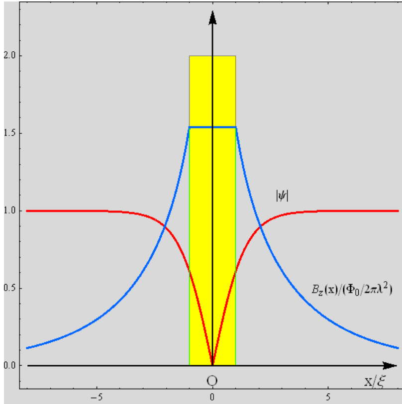
Fig. Plot of the magnetic induction B(r) = \frac{\Phi_0}{2\pi\lambda^2} K_0\left(\frac{x}{\lambda}\right) and the order parameter |\psi(x)|/\psi_\infty as a function of x/\xi . We use the GL parameter as \kappa = \lambda/\xi = 4 .
