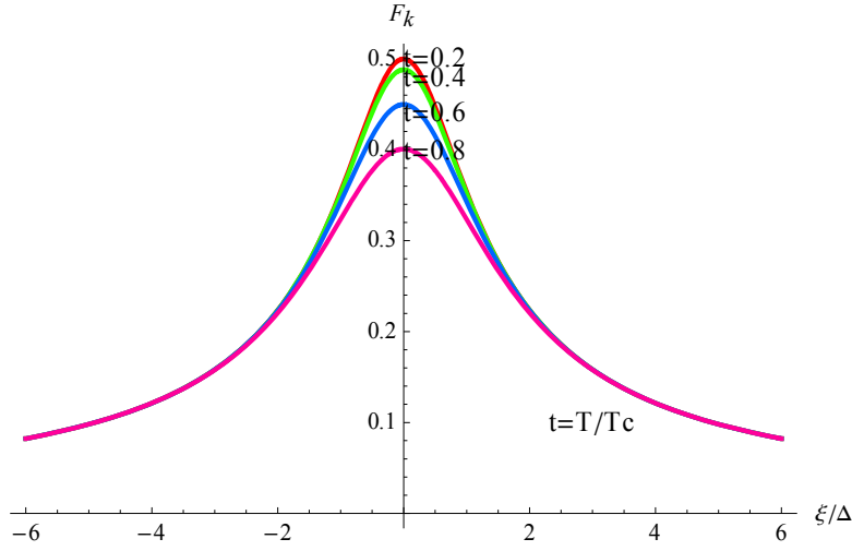
Fig. Plot of the condensation amplitude F as a function of \xi/\Delta . \xi/\Delta . t is the reduced temperature; t = T/T_c . t = 0.2, 0.4, 0.6, and 0.8 . We assume that the energy gap is independent of t .
