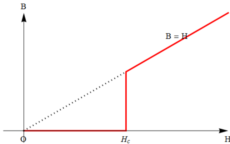
Fig. B vs an external field H for the type-I superconductor. B is the magnetic induction. B = H + 4\pi M .
