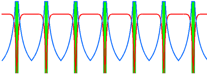
Fig. One dimensional Abrikosov-type structure of vortices.. The red line shows the distribution of the normalized order parameter and the blue line shows the distribution of the magnetic induction (the internal magnetic field). The center of each vortex is denoted by the green lines.
