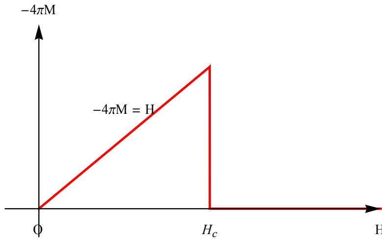
Fig. (-4\pi M) vs an external field H for the type-I superconductor. M is the magnetization
