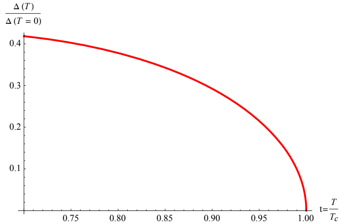
Fig. Plot of f(t) = \Delta(T)/(3.06326k_B T_c) as a function of reduced temperature t = T/T_c .
