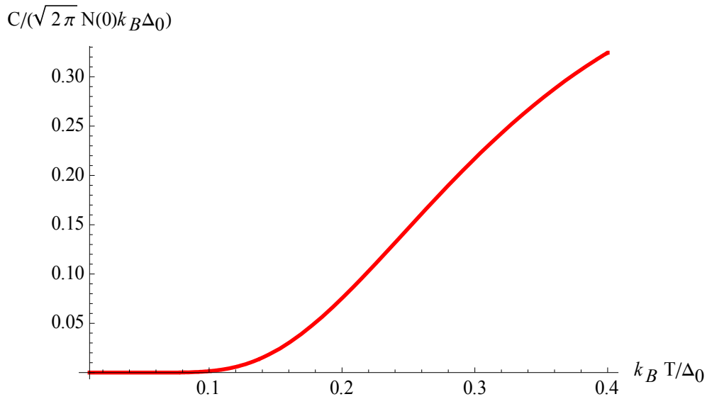
Fig. Plot of C_{es} / [\sqrt{2\pi} N(0) k_B \Delta_0] as a function of k_B T / \Delta_0 for T \ll \Delta_0 / k_B .
